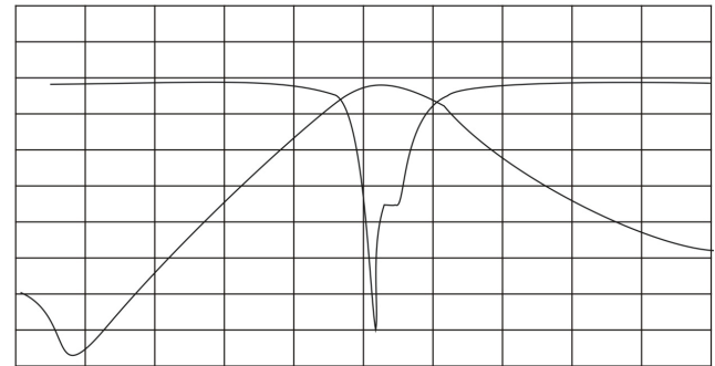
DFC1575P0002 Transmission & Reflection
